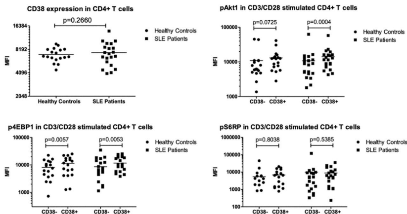
Figure 3. In SLE patients' CD38 + CD4 + T cells compared to CD38 - CD4 + T cells, pAkt1 ( p=0.0004 ) and pEBP1 ( p=0.0053 ) are increased.
